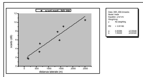
Figure 4, Correlation SEL differences-distance
