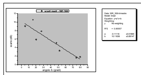
Figure 5, Correlation SEL differences -elevation angle
