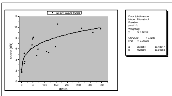
Figure 6, Correlation SEL differences-lateral distance/elevation angle
