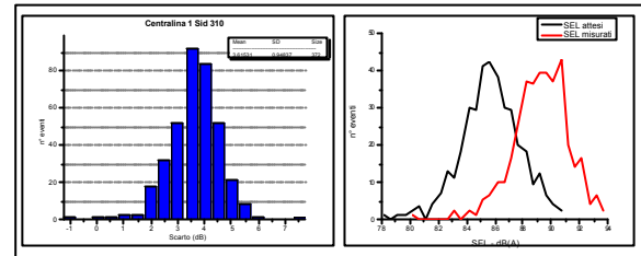
Figure 3, Differences between calculated and measured data statistical distribution
