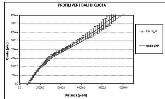
Figure 1, Vertical dispersion of MD 80 radar tracks and user profile
