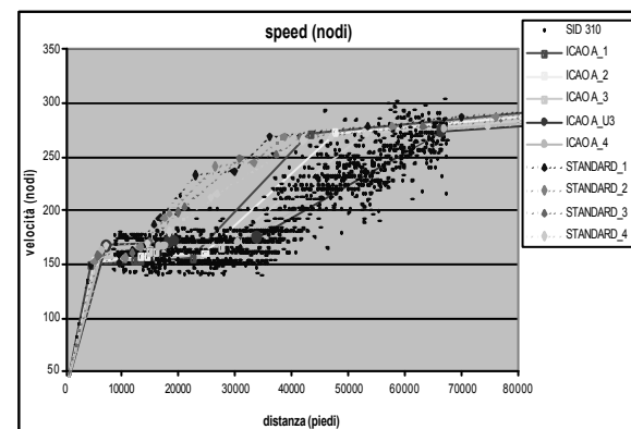
Figure 2, Comparison of several type of INM outputs and RDL 310 radar data speed profile
